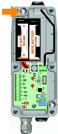
TRANSMITTER
